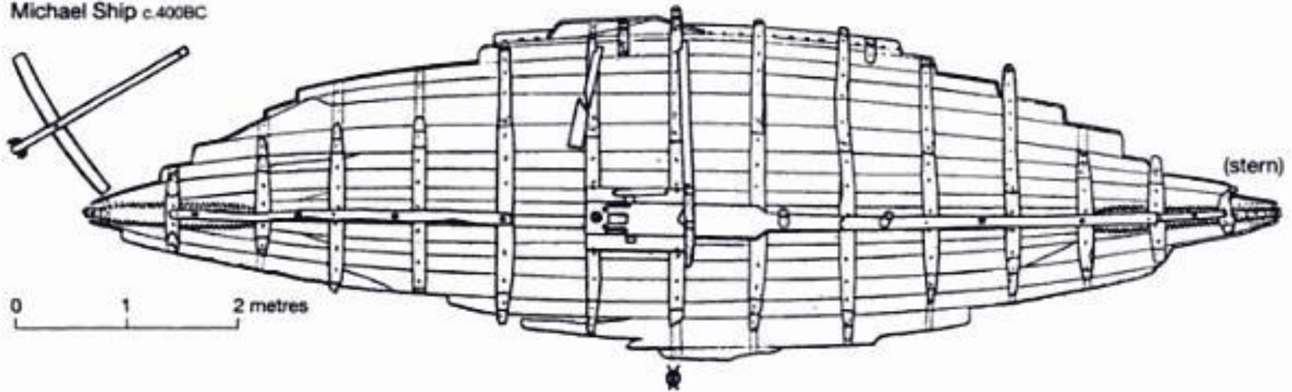
Plan of the Ma'agan-Michael wreck (Yak Kahanov).
